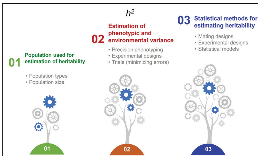
Fig. 4: Enhancing trait heritability
